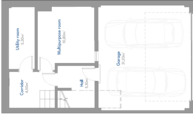
Basement Floor
